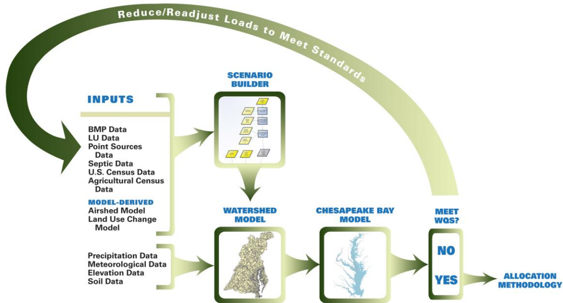
Figure 5-7. Chesapeake Bay TMDL modeling framework.
